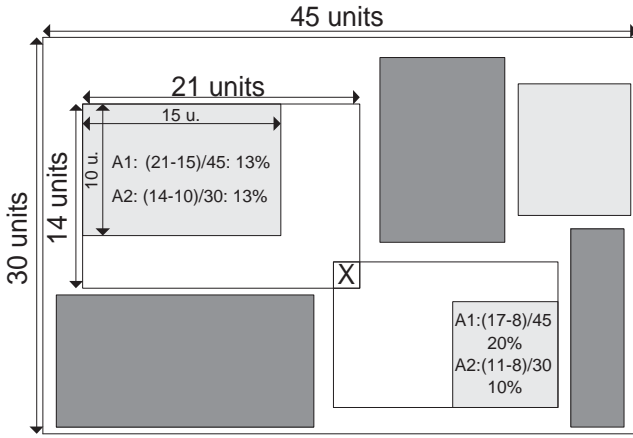
Figure 1: Two rules are candidate to describe a new example but both exceed the maximum generalization ( \kappa=10\% ) in attribute A1.
