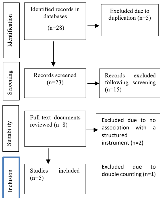
Figure 1. PRISMA-ScR Flowchart
